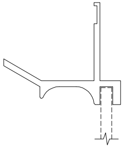
RETRO HEAD DRIP USED WITH RETRO SURROUND; for: 1000, 1500, 2000, 2500, 3000 SERIES WINDOWS
